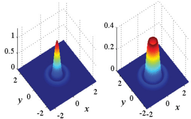
FIG. 2. (Color online) Density profiles of spin-up and -down components for the single-particle ground state \phi_{j_z=\frac{1}{2}} with the parameter values of \alpha = 4 and \rho = \gamma = 0 . Only the spin-down component carries a vortex. The corresponding density profile for \phi_{j_z=-\frac{1}{2}} is obtained by interchanging the spin indices. Here we use the length unit defined by the harmonic trap.
