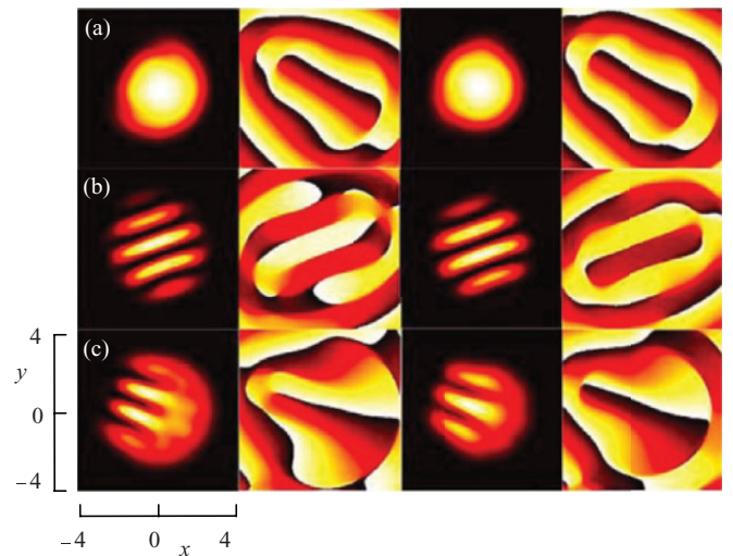
FIG. 6. (Color online) From left to right: the density and phase profiles of spin-up and -down components with the parameter values of \alpha = 2.5 , \beta = 40 , and \gamma = 0 . (a) c = 0.6 and \rho = 0.2 ; a plane-wave-like state is obtained with a distorted phase pattern; (b) c = 1.2 and \rho = 0.2 ; the spin-spiral condensate is favored; (c) c = 1.2 and \rho = 0.5 ; the condensate exhibits an intermediate configuration between those of (a) and (b). The color scales for the density and phase distributions are the same as those in Fig. 4. The unit of length for the figures is l .
