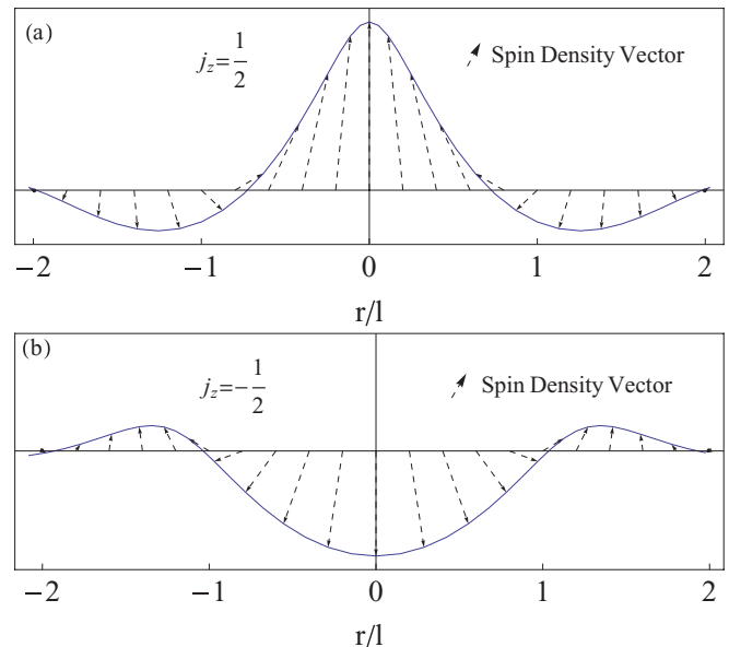
FIG. 3. (Color online) Spin-density vector distributions along the x axis lie in the xz plane as shown in (a) j_z = \frac{1}{2} and (b) j_z = -\frac{1}{2} with \alpha = 4 and \rho = \gamma = 0 . They are time-reversal counterparts to each other, and both exhibit the Skymion-type texture configuration.
